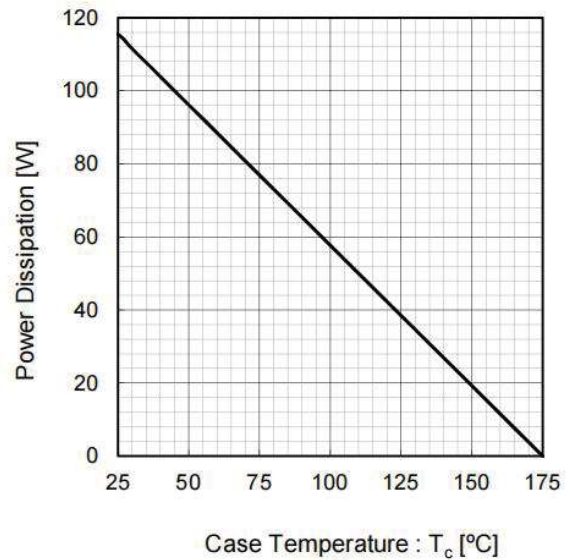
Fig.6 Power Dissipation
