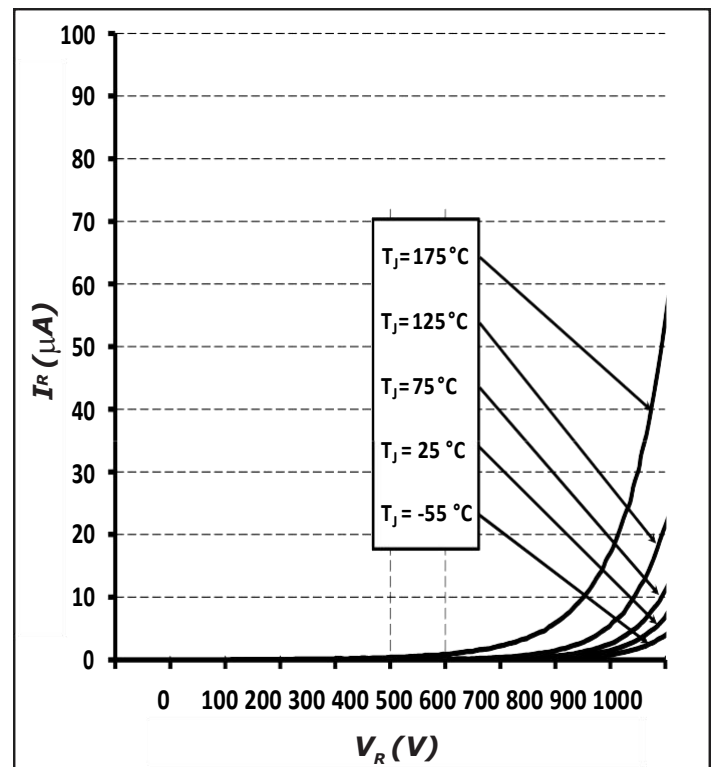
Figure 2. Reverse Characteristics
