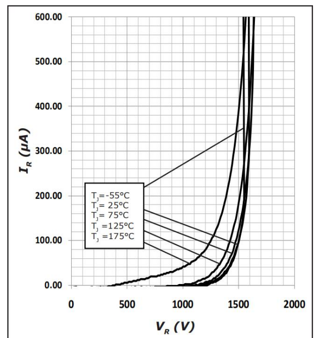
Figure 2. Reverse Characteristics
