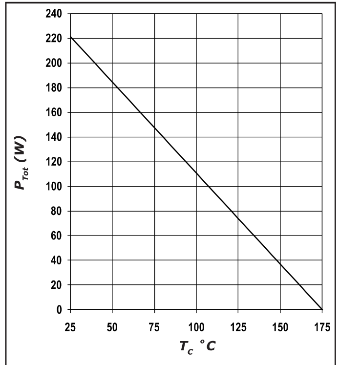
Figure 4. Power Derating
