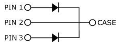
TO-247-3
