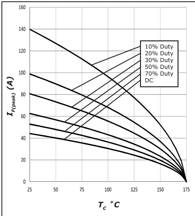
Figure 3. Current Derating
