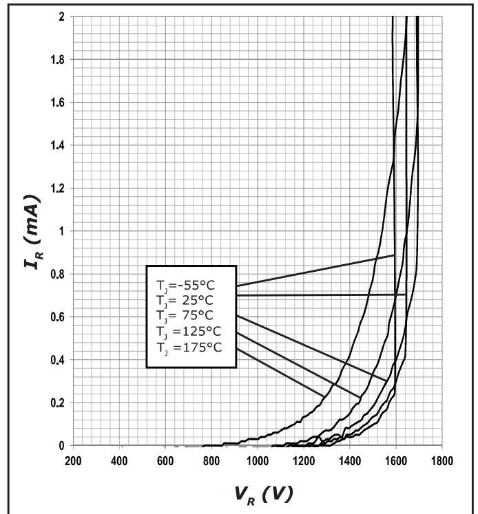
Figure 2. Reverse Characteristics
